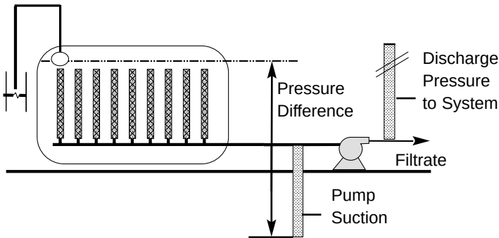
Figure 3-B Vacuum Filter
