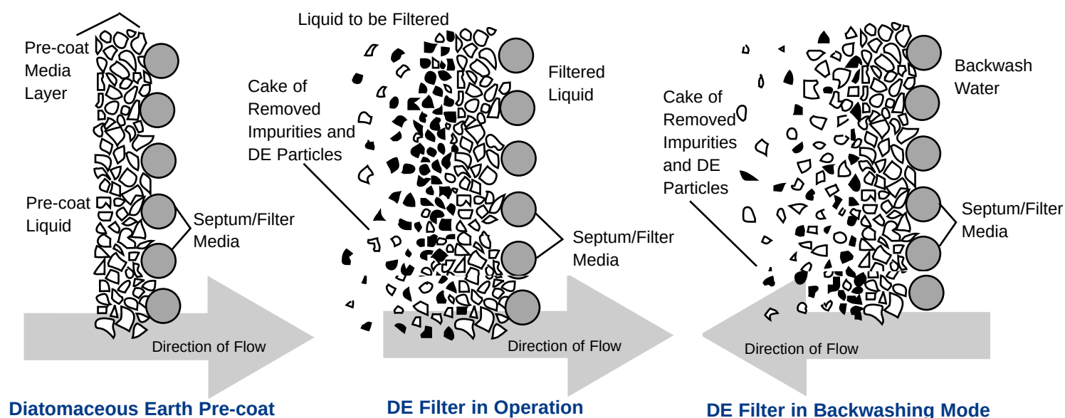
Figure 1 Diatomaceous Earth Filter
