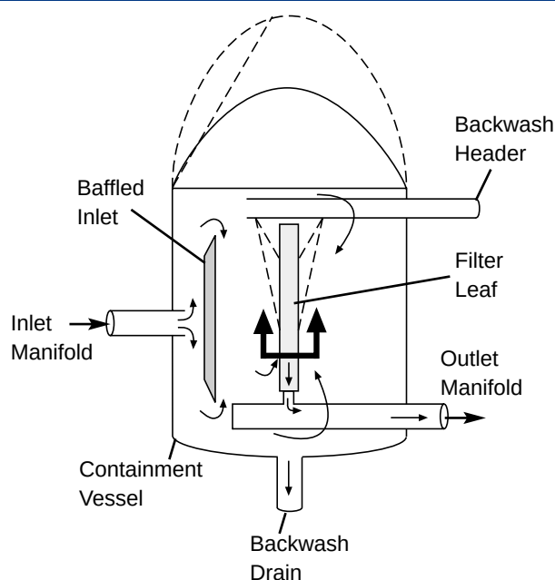
Figure 2 Elements of a Flat Leaf Filter
